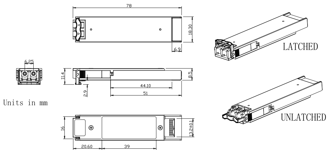
XFP Transceiver (dimensions are in mm)
